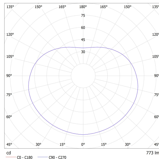
Luminaire: Lucis ZKS.L2.200.X POLARIS ZKS LED Lamps: 1 x LED G6
