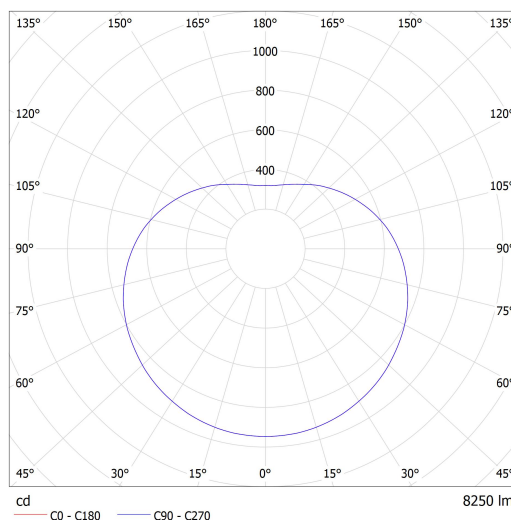
Luminaire: Lucis ZT.P4.600.X POLARIS ZT LED Lamps: 1 x LED G6
