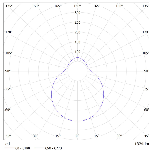
Luminaire: Lucis S24.L4.D350 DAPHNE LED Lamps: 1 x LED G6
