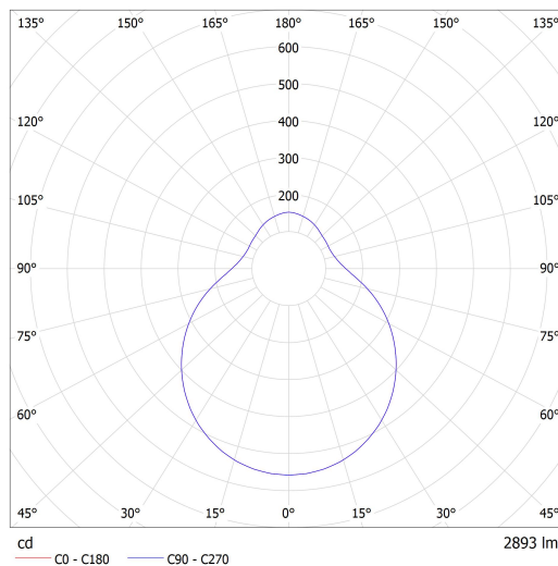
Luminaire: Lucis S43.L5.D550 DAPHNE LED Lamps: 1 x LED G6
