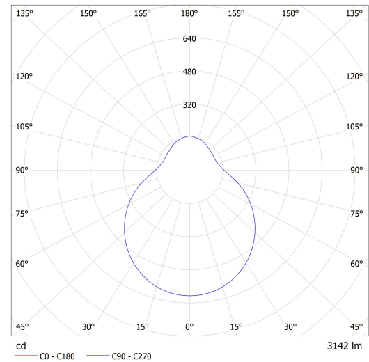
Luminaire: Lucis S43.L6.D550 DAPHNE LED Lamps: 1 x LED G6
