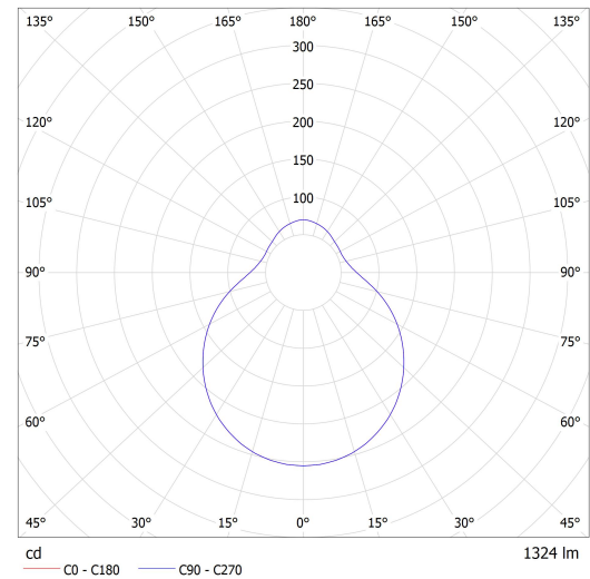
Luminaire: Lucis PS13.L4.D350 DAPHNE LED Lamps: 1 x LED G6
