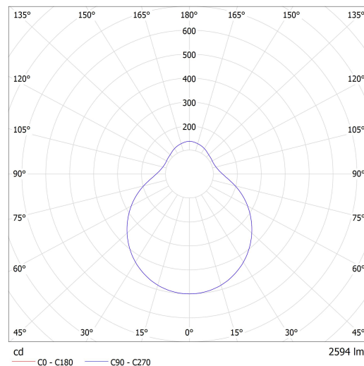
Luminaire: Lucis PS13.L6.D450 DAPHNE LED Lamps: 1 x LED G6
