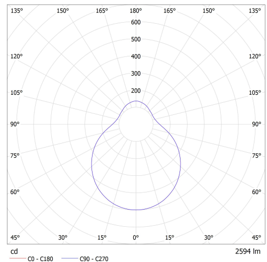
Luminaire: Lucis ZL3.L4.D451.X DAPHNE LED Lamps: 1 x LED G6
