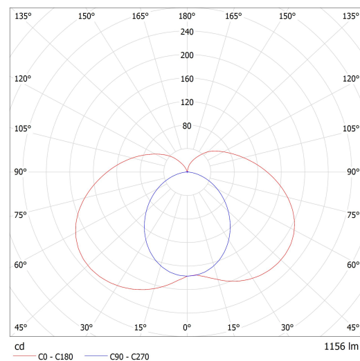
Luminaire: Lucis AU3.L1.350.X AULA LED Lamps: 1 x LED G6
