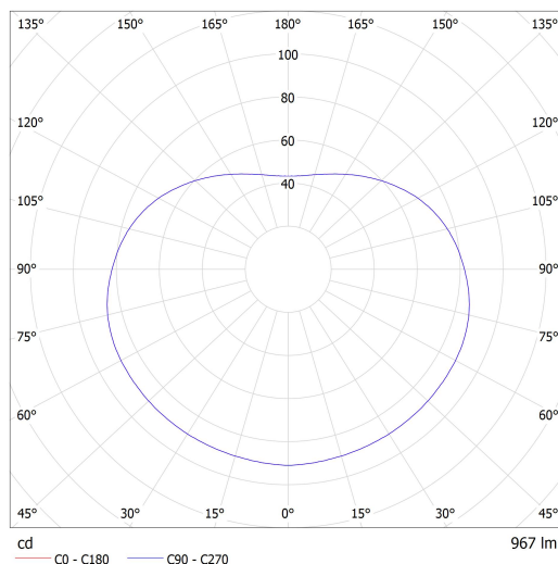
Lucis ZTR.L1.200.X POLARIS ZTR LED / LDC (Polar)
