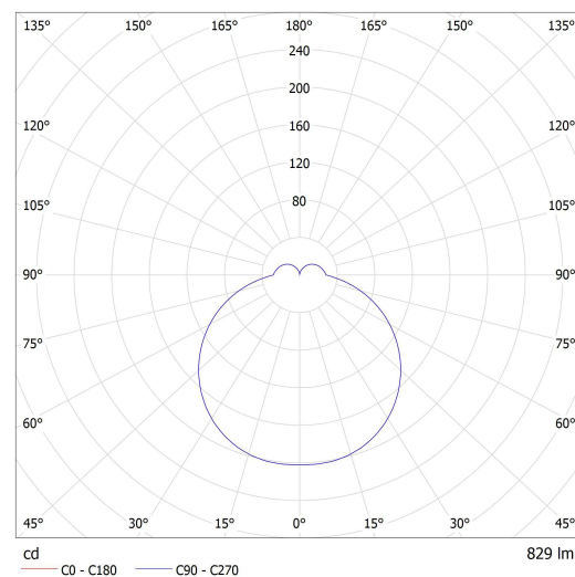
Lucis BS14.K1.N14.X NOMIA LED / LDC (Polar)
