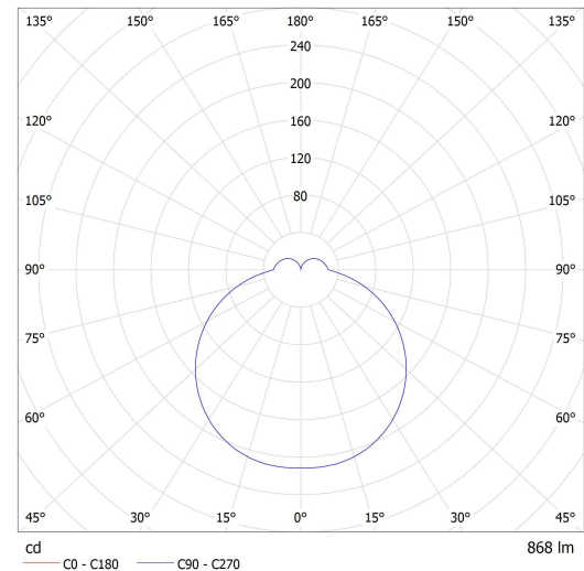
Lucis BS14.K2.N14.X NOMIA LED / LDC (Polar)
