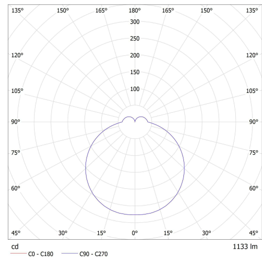
Lucis BS24.K3.N24.X NOMIA LED / LDC (Polar)
