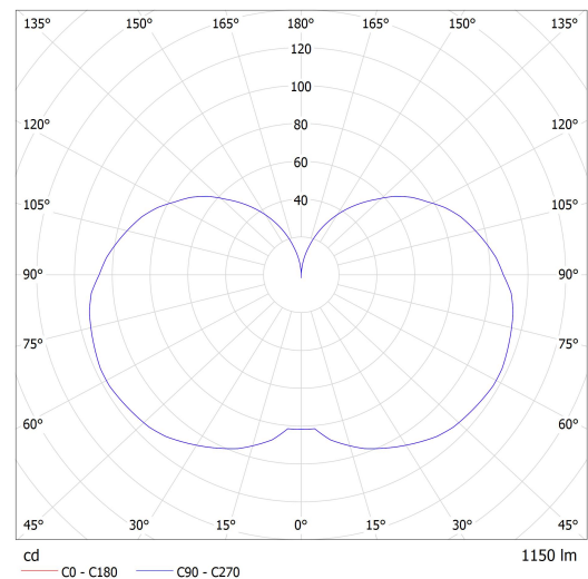
Luminaire: Lucis BS19.L1.R19.X RETRO LED Lamps: 1 x LED G66
