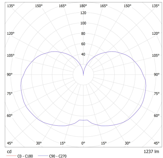
Luminaire: Lucis BS19.L2.R19.X RETRO LED Lamps: 1 x LED G6
