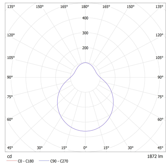
Luminaire: Lucis ZL3.L5.D451.X DAPHNE LED Lamps: 1 x LED G6
