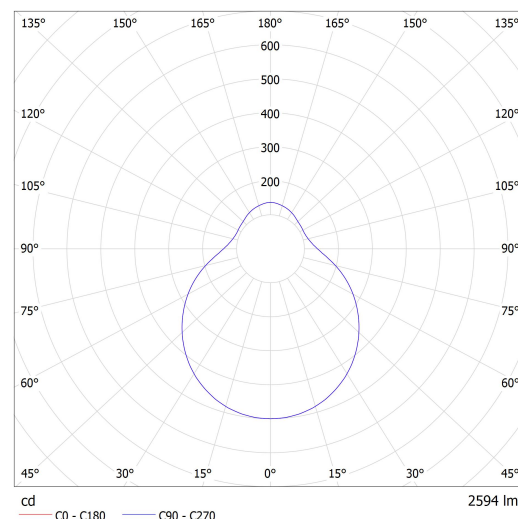
Luminaire: Lucis ZL3.L6.D551.X DAPHNE LED Lamps: 1 x LED G6
