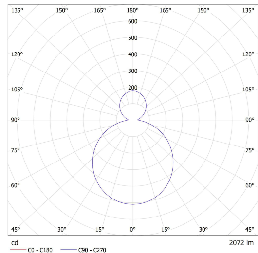
Lucis ZT.K1.R450.X RONDO LED / LDC (Polar)
