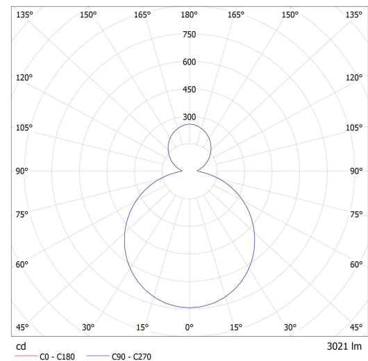
Lucis ZT.K1.R550.X RONDO LED / LDC (Polar)
