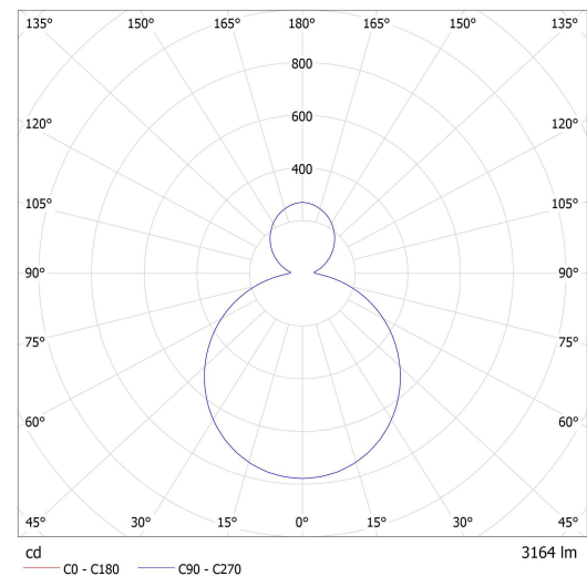
Lucis ZT.K2.R550.X RONDO LED / LDC (Polar)
