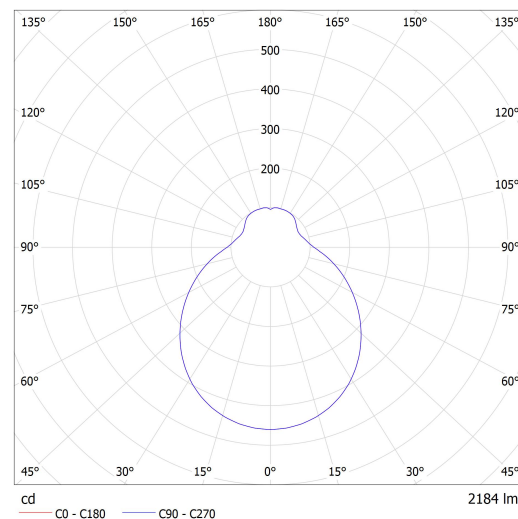
Luminaire: Lucis S37.L3.T14 CHARON LED Lamps: 1 x LED G6
