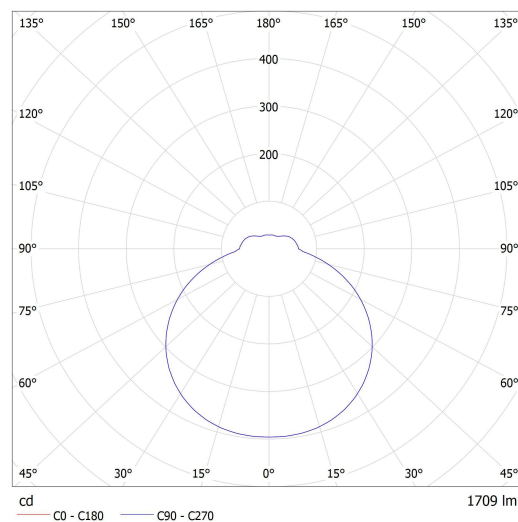
Lucis S26.K1.TEZ2 TENDO LED / LDC (Polar)
