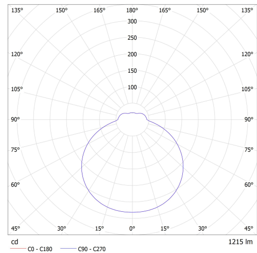
Lucis S26.K3.TEZ2 TENDO LED / LDC (Polar)
