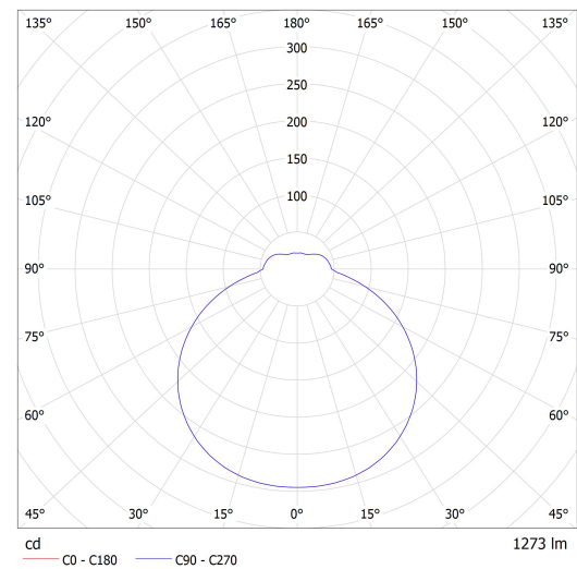
Lucis S26.K4.TEZ2 TENDO LED / LDC (Polar)
