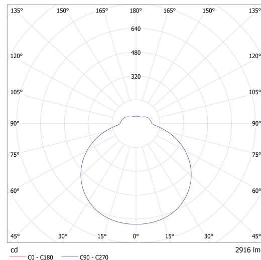
Lucis S44.K3.TEZ4 TENDO LED / LDC (Polar)
