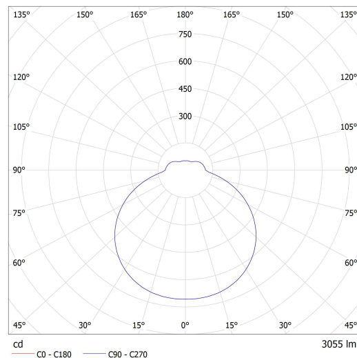
Lucis S44.K4.TEZ4 TENDO LED / LDC (Polar)
