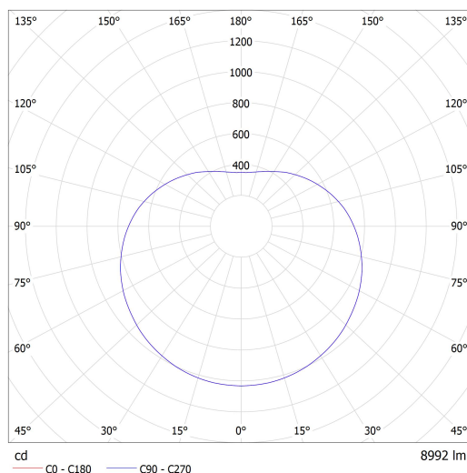
Lucis ZKS.P8.400.X POLARIS ZKS.P LED / LDC (Polar)
