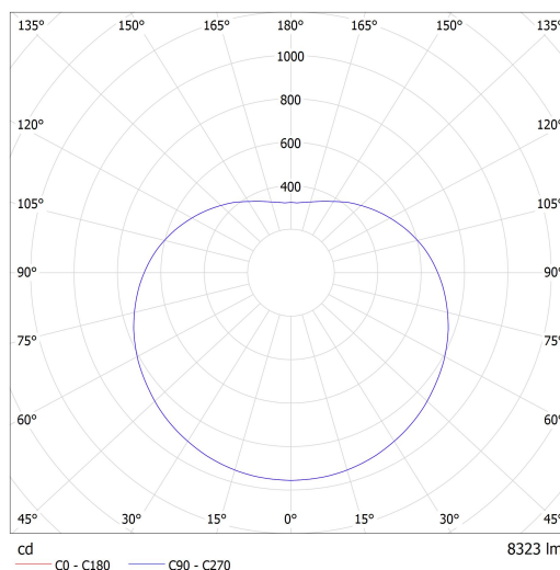
Luminaire: Lucis ZKS.P7.400.X POLARIS ZKS.P LED Lamps: 1 x LED G6
