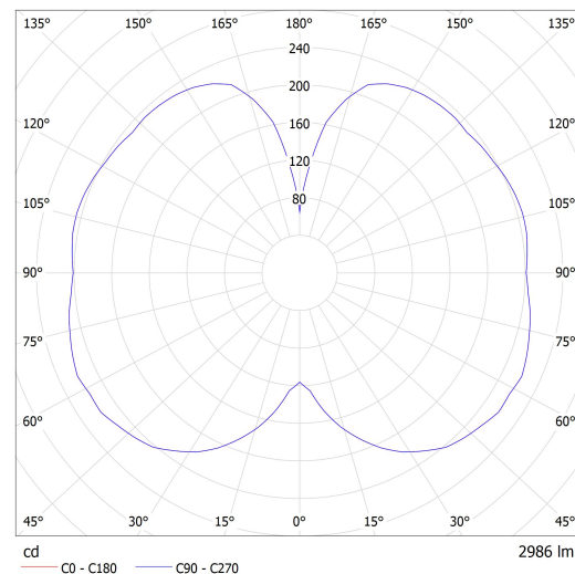
Lucis ZK.L3B.M500 MAIA LED / LDC (Polar)
