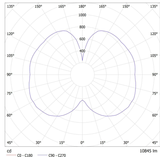
Lucis ZK.L1B.M800 MAIA LED / LDC (Polar)
