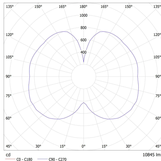
Lucis ZK.L1B.M800 MAIA LED / LDC (Polar)
