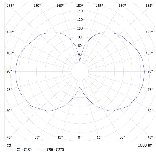
Lucis ZK.L1B.M320 PA MAIA LED / LDC (Polar)
