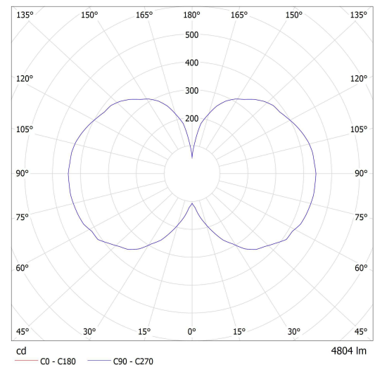
Lucis ZK.L1B.M620 PA MAIA LED / LDC (Polar)
