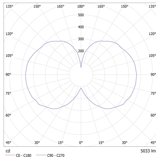
Lucis ZK.L2B.M620 PA MAIA LED / LDC (Polar)
