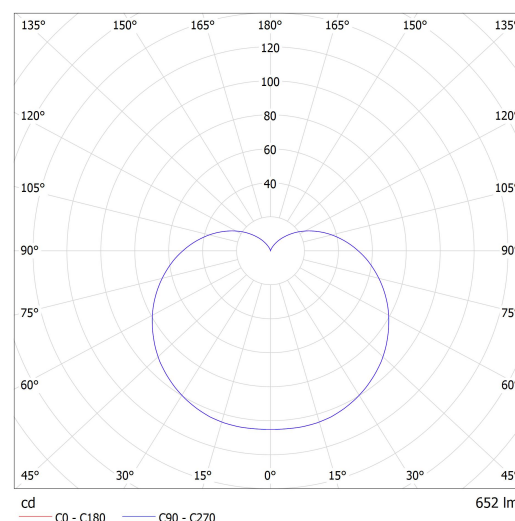
Luminaire: Lucis ZL.L1.C20.X CAPSULE LED Lamps: 1 x LED G6
