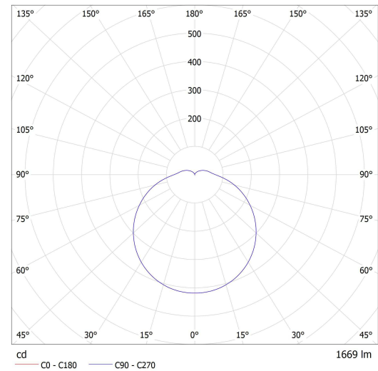
Lucis BS24.K2.P24.X PRIMA LED / LDC (Polar)
