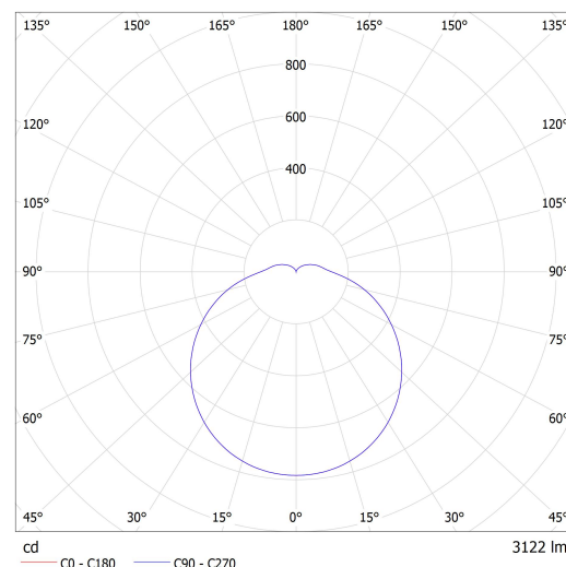
Lucis BS34.K2.P34.X PRIMA LED / LDC (Polar)
