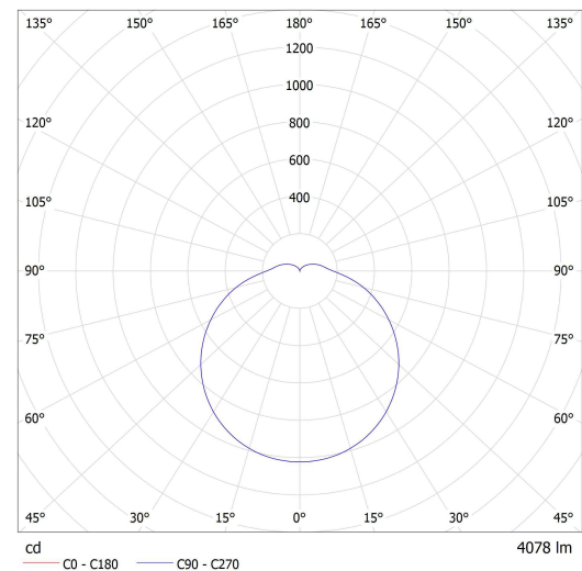
Lucis BS44.K2.P44.X PRIMA LED / LDC (Polar)
