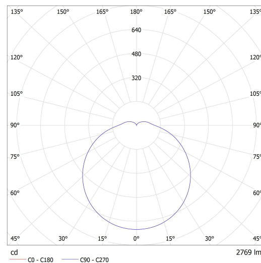
Lucis BS44.K4.P44.X PRIMA LED / LDC (Polar)
