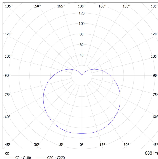
Luminaire: Lucis SR.L2.S200.X SEMILUNA LED Lamps: 1 x LED G6
