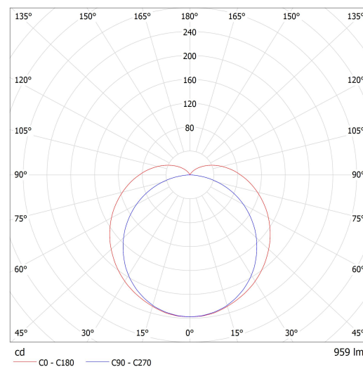
Luminaire: Lucis PS2.L4.X CASTOR LED Lamps: 1 x LED G6
