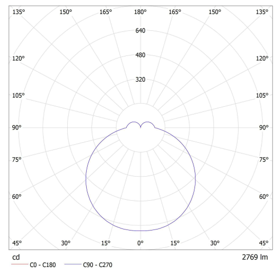
Lucis BS44.K4.N44.X NOMIA LED / LDC (Polar)
