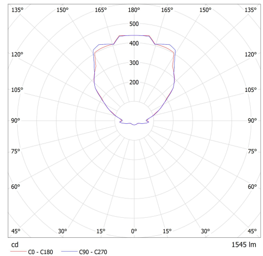
Lucis N2.K1.60 GLOU / LDC (Polar)
