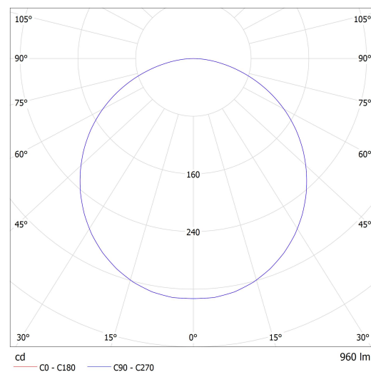
Lucis SR1.K1.02.X OMNIA LED / LDC (Polar)
