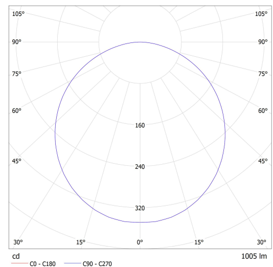
Lucis SR1.K2.O2.X OMNIA LED / LDC (Polar)
