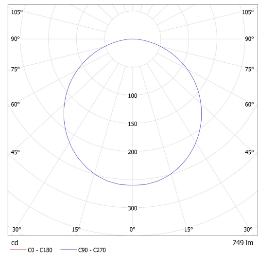
Lucis ZT2.6.K2.O2.X_pc(2) OMNIA LED / LDC (Polar)
