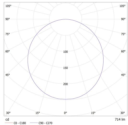
Lucis ZT2.12.K1.02.X_pc(2) OMNIA LED / LDC (Polar)
