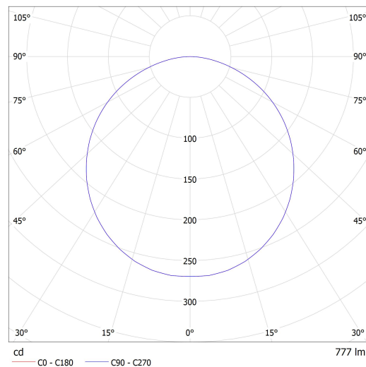
Luminaire: Lucis ZT4.K2.O2.X_pc(4) OMNIA LED Lamps: 1 x LED G5
