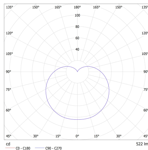
Luminaire: Lucis ZL.L2.C15.X CAPSULE LED Lamps: 1 x LED G6
