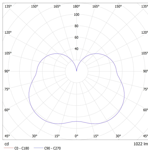
Luminaire: Lucis ZL1.IC.K1.150.X IZAR C LED Lamps: 1 x LED 103/73-G5
